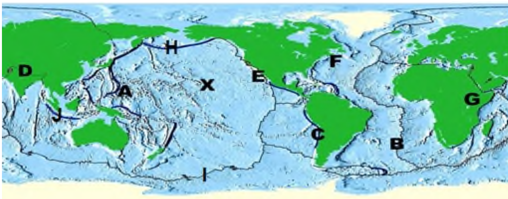
Tectonic Plate Boundary Map
